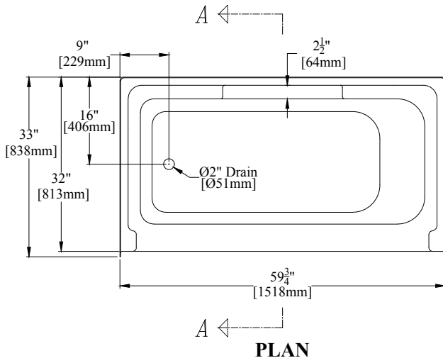
59 3/4" [1518mm] Bathtub w/ Removable Access Panel
